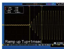
Mode=Time, T_{up}=1\text{msec} , V_{AC}=100\text{V} , \text{Freq}=50\text{Hz} , Ramp output=on.
